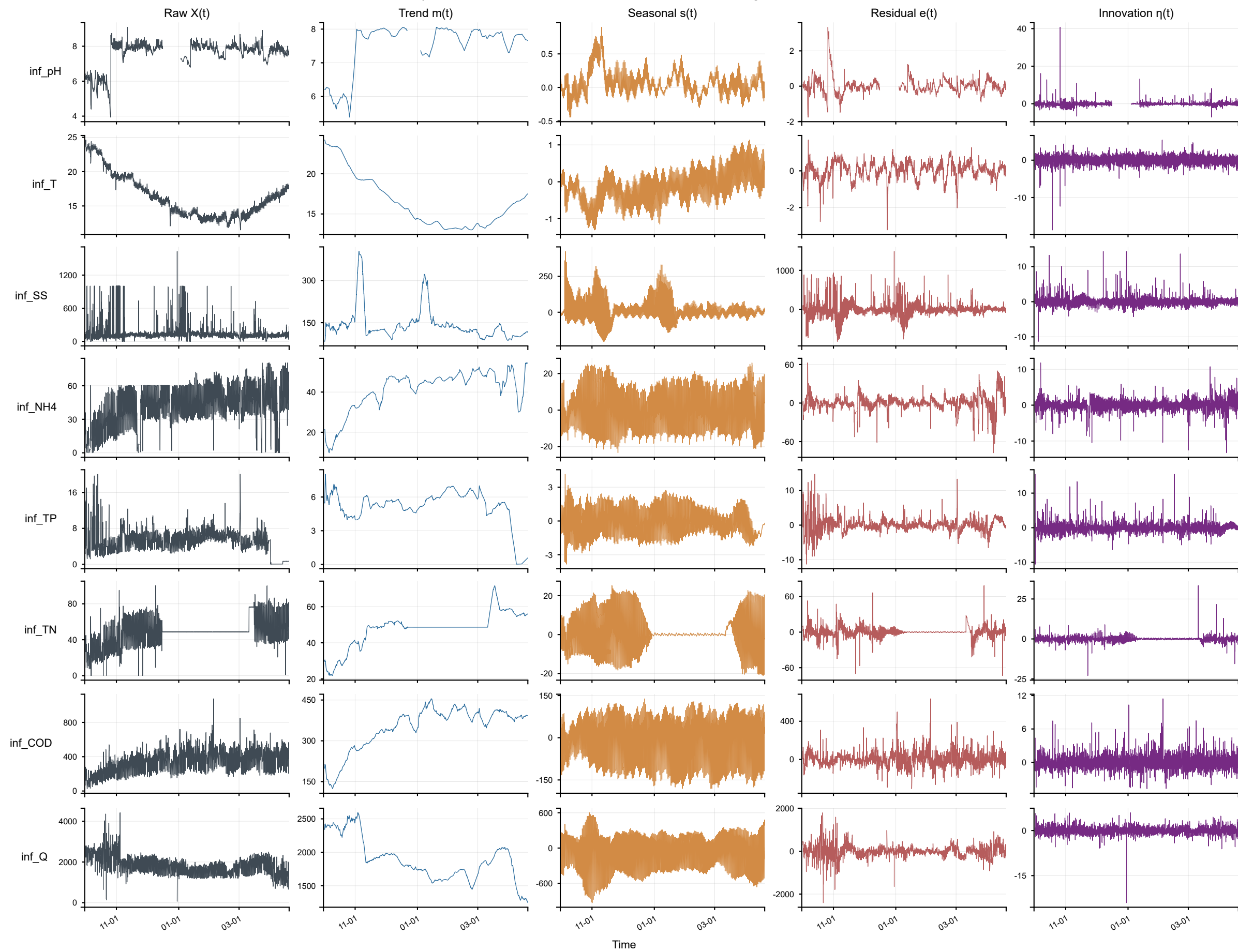
Influent water-quality variables — trend/seasonal/residual/innovation grid [2025-10-01~2026-04-19]
